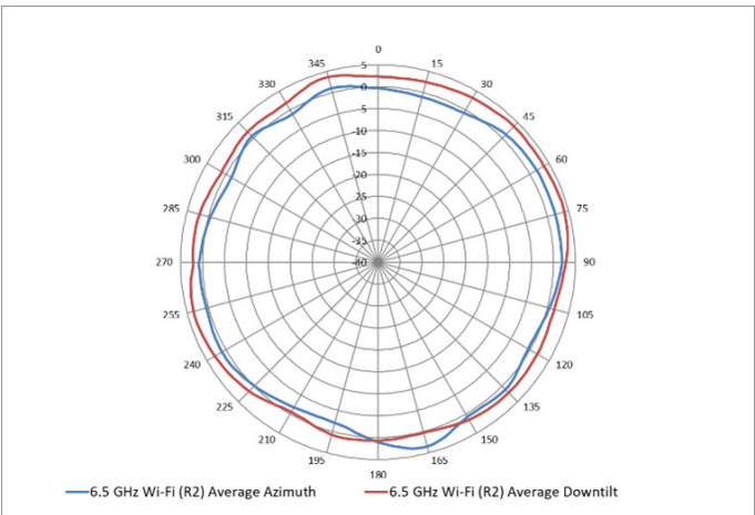
Figure 3. 6.5 GHz Wi-Fi antenna patterns (horizontal)
