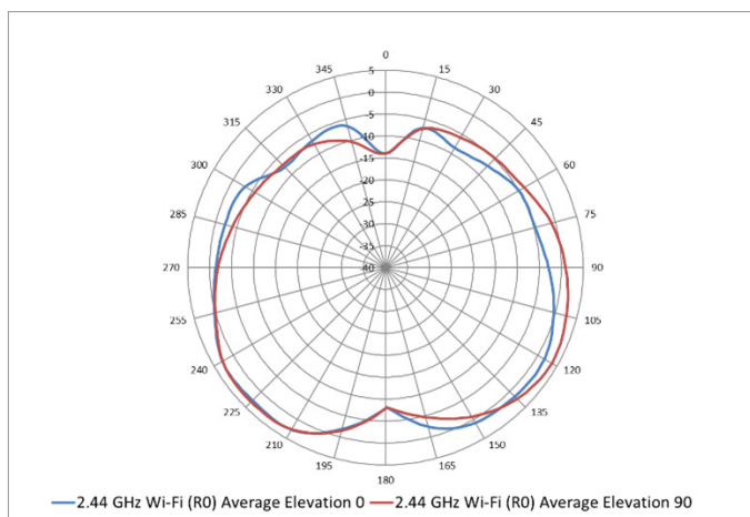
Figure 4. 2.44 GHz Wi-Fi antennas patterns (vertical)
